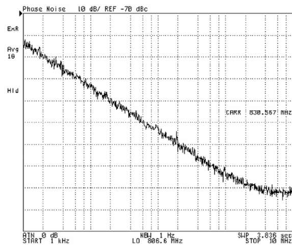
Fig. 12: Example of VCO Phase Noise Measurement Using the 4352S
