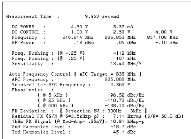
Fig. 18: Measurement Example on the VCO Production Line Using the 4352S
