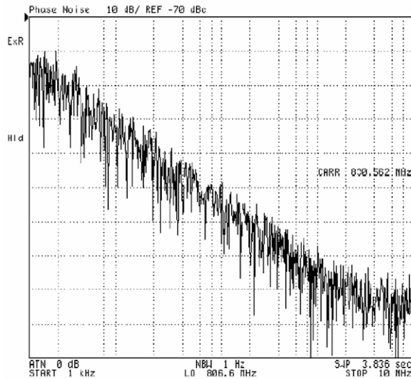
Fig. 4: Phase Noise Measurement Results without Averaging
