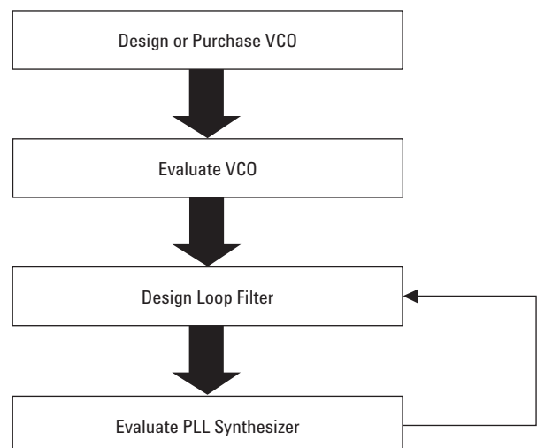
Fig. 2: PLL Frequency Synthesizer Design Flow
