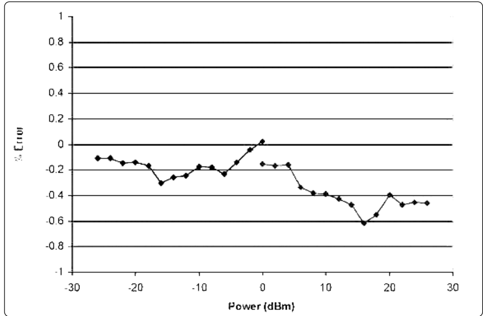
Typical E9300H/01H power linearity at 25°C, after zero and calibration, with associated measurement uncertainty
