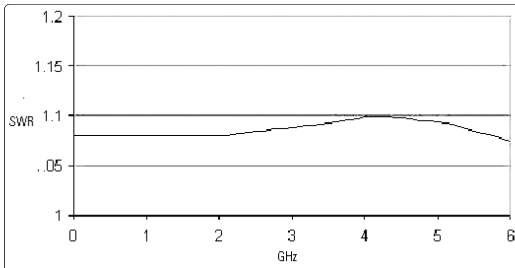
Typical SWR, 9kHz to 6 GHz, (25°C ± 10°C) for E9304A sensors
