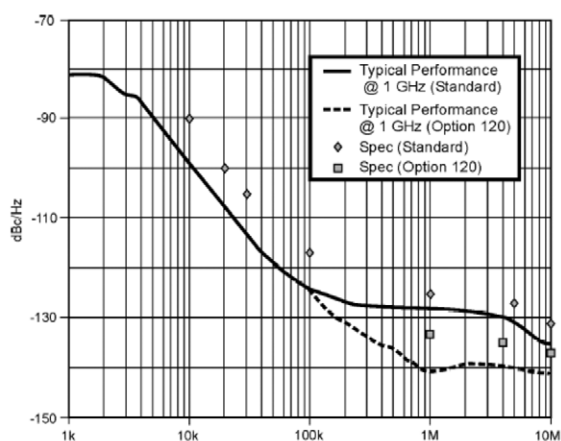
Figure 1. Typical ESA-E Series performance at 1 GHz
