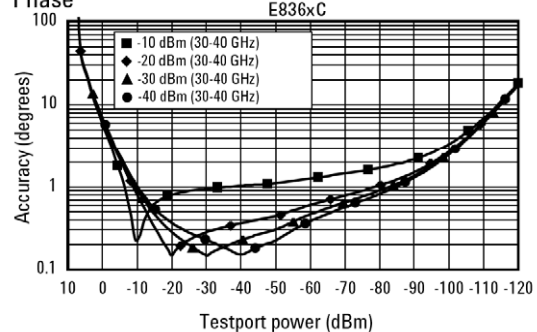
Phase
