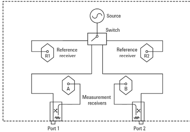
Configuration test set (Option 014)
